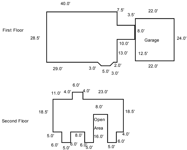
Subject's Floorplan/Layout
